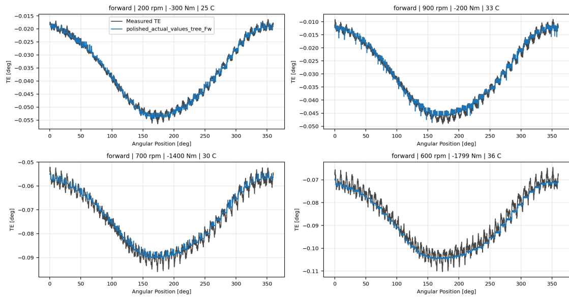
polished_actual_values_tree_Fw measured-versus-predicted TE collage
