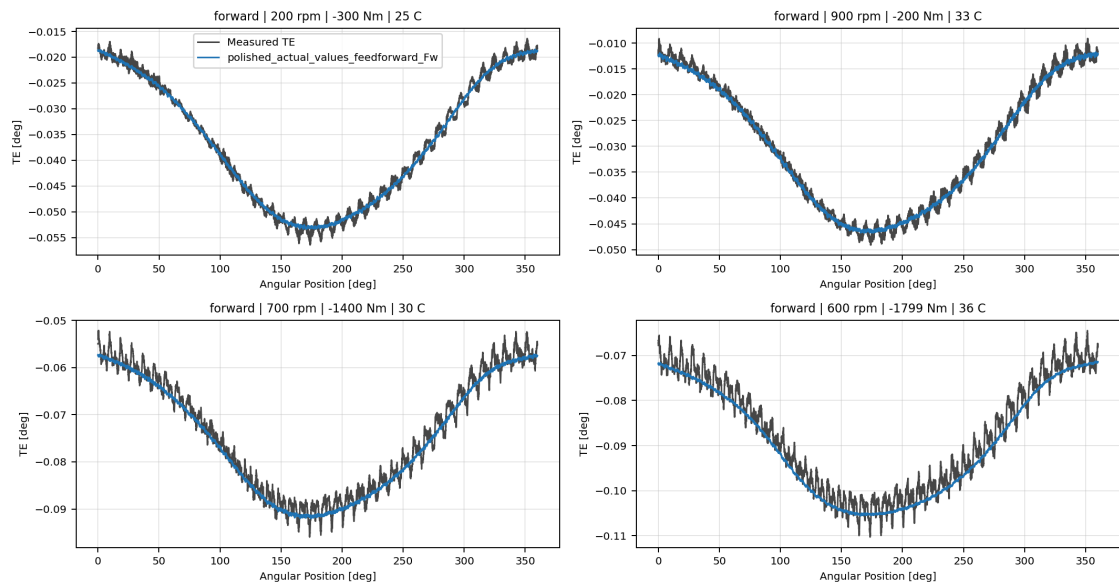
polished_actual_values_feedforward_Fw measured-versus-predicted TE collage
