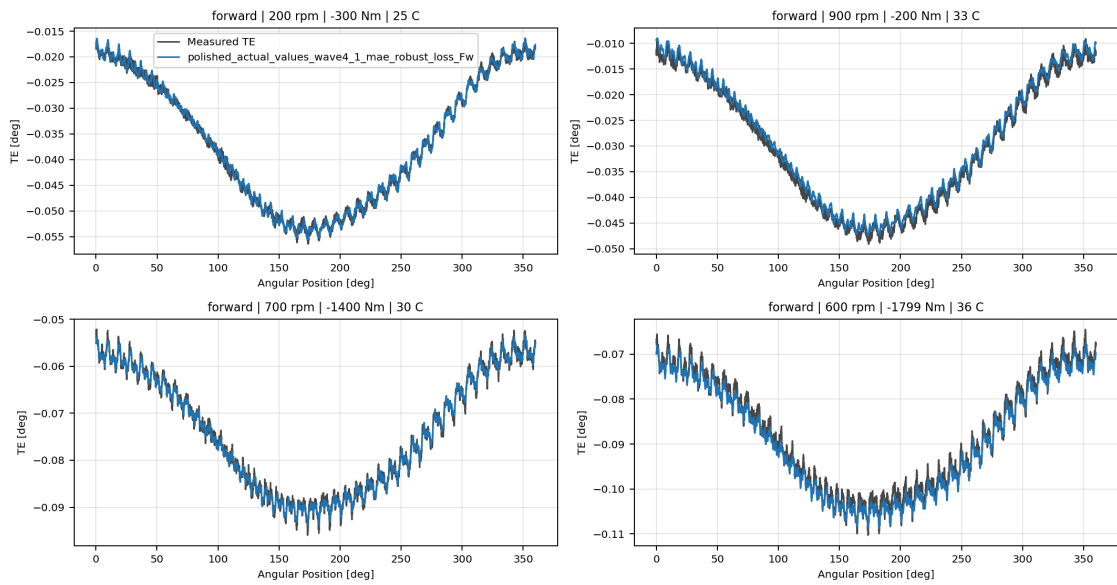
polished_actual_values_wave4_1_mae_robust_loss_Fw measured-versus-predicted TE collage
