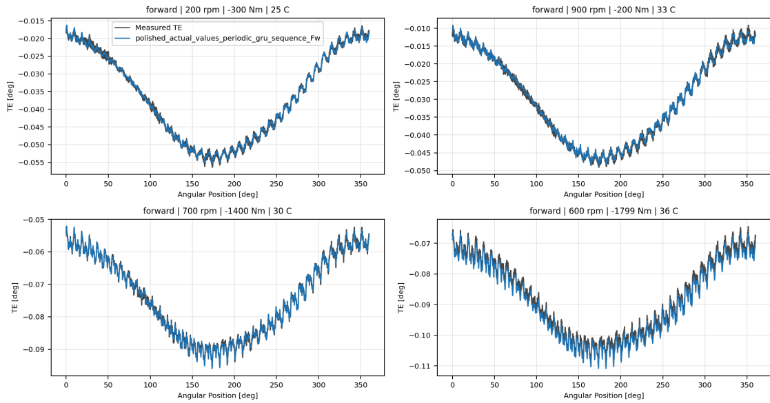
polished_actual_values_periodic_gru_sequence_Fw measured-versus-predicted TE collage
