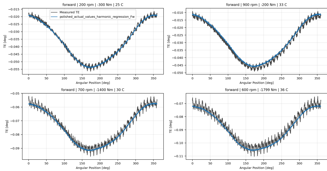
polished_actual_values_harmonic_regression_Fw measured-versus-predicted TE collage
