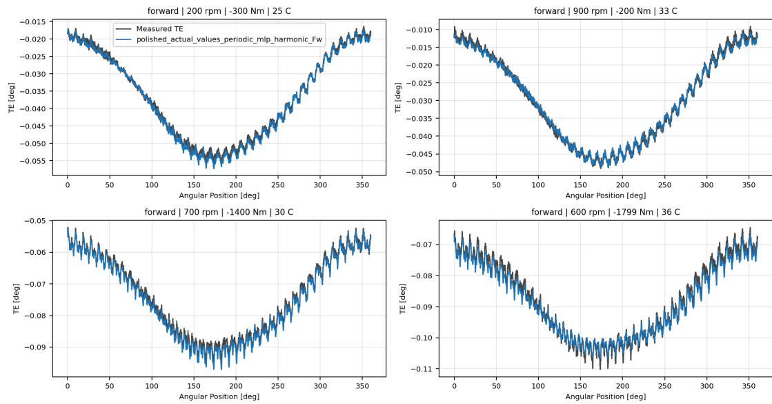
polished_actual_values_periodic_mlp_harmonic_Fw measured-versus-predicted TE collage
