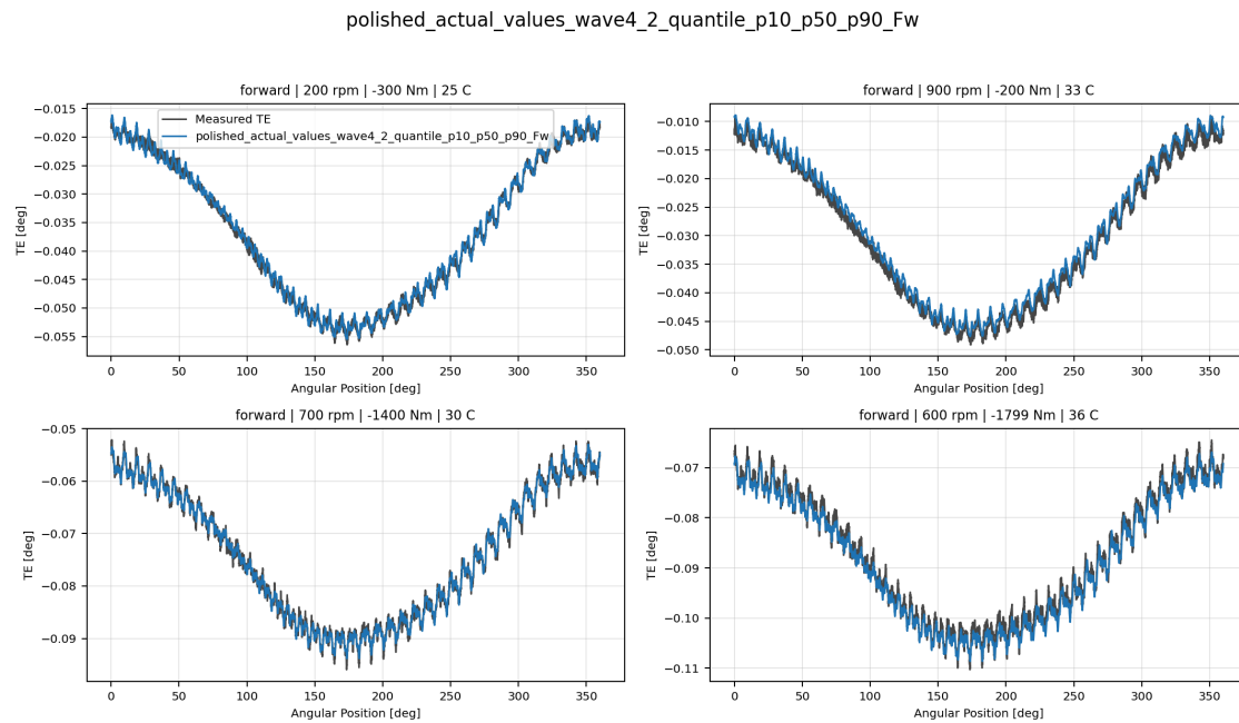
polished_actual_values_wave4_2_quantile_p10_p50_p90_Fw measured-versus-predicted TE collage
